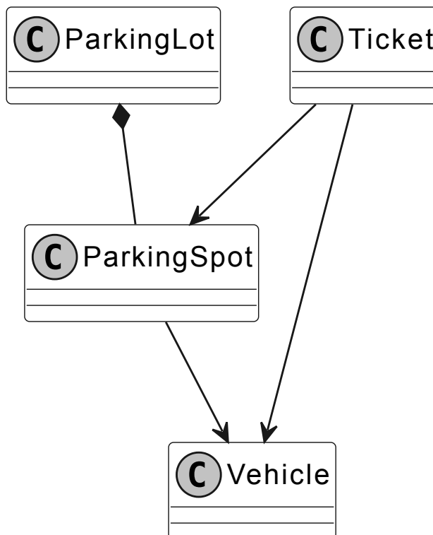
Class diagram of Parking Lot
